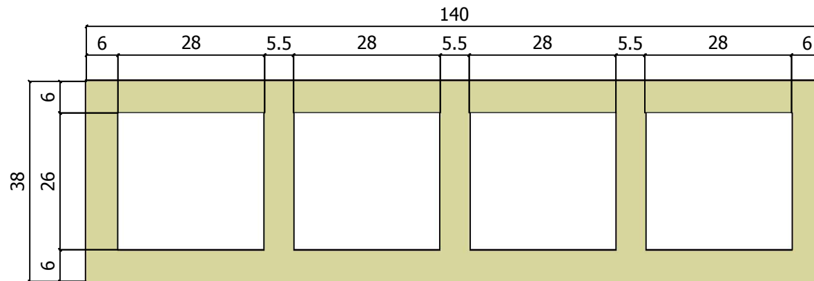
FRONT ELEVATION RESGC020616N*
