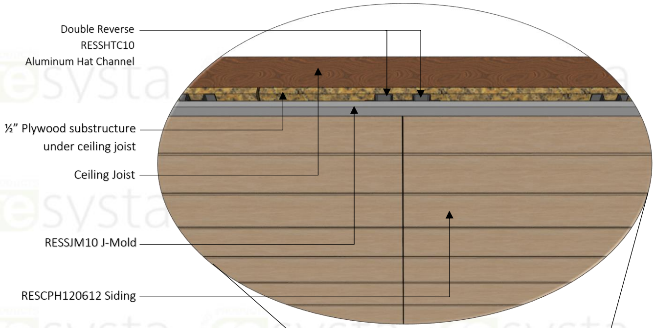
ISOMETRIC DETAIL SIDING BOARD ON SOFFIT
