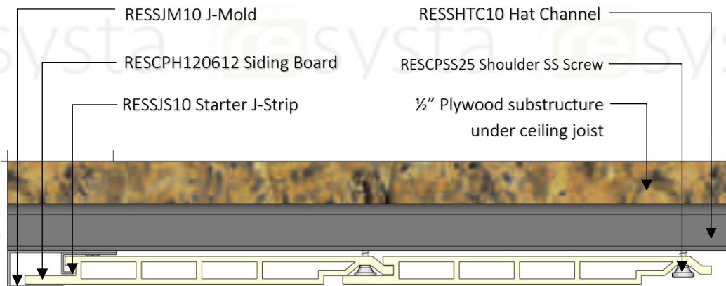
SECTION DETAIL SIDING BOARD ON SOFFIT
