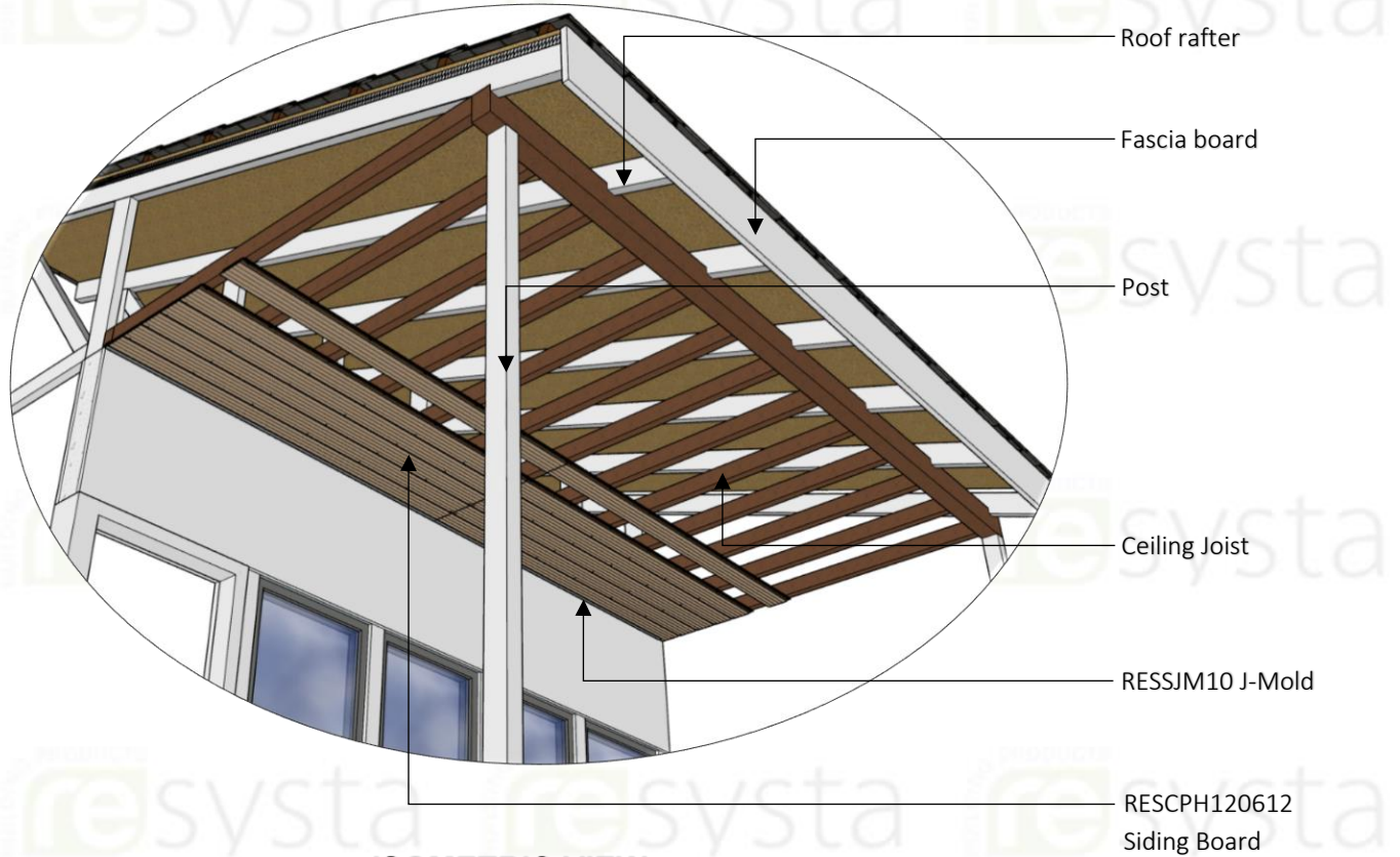
ISOMETRIC VIEW SIDING BOARD ON SOFFIT
