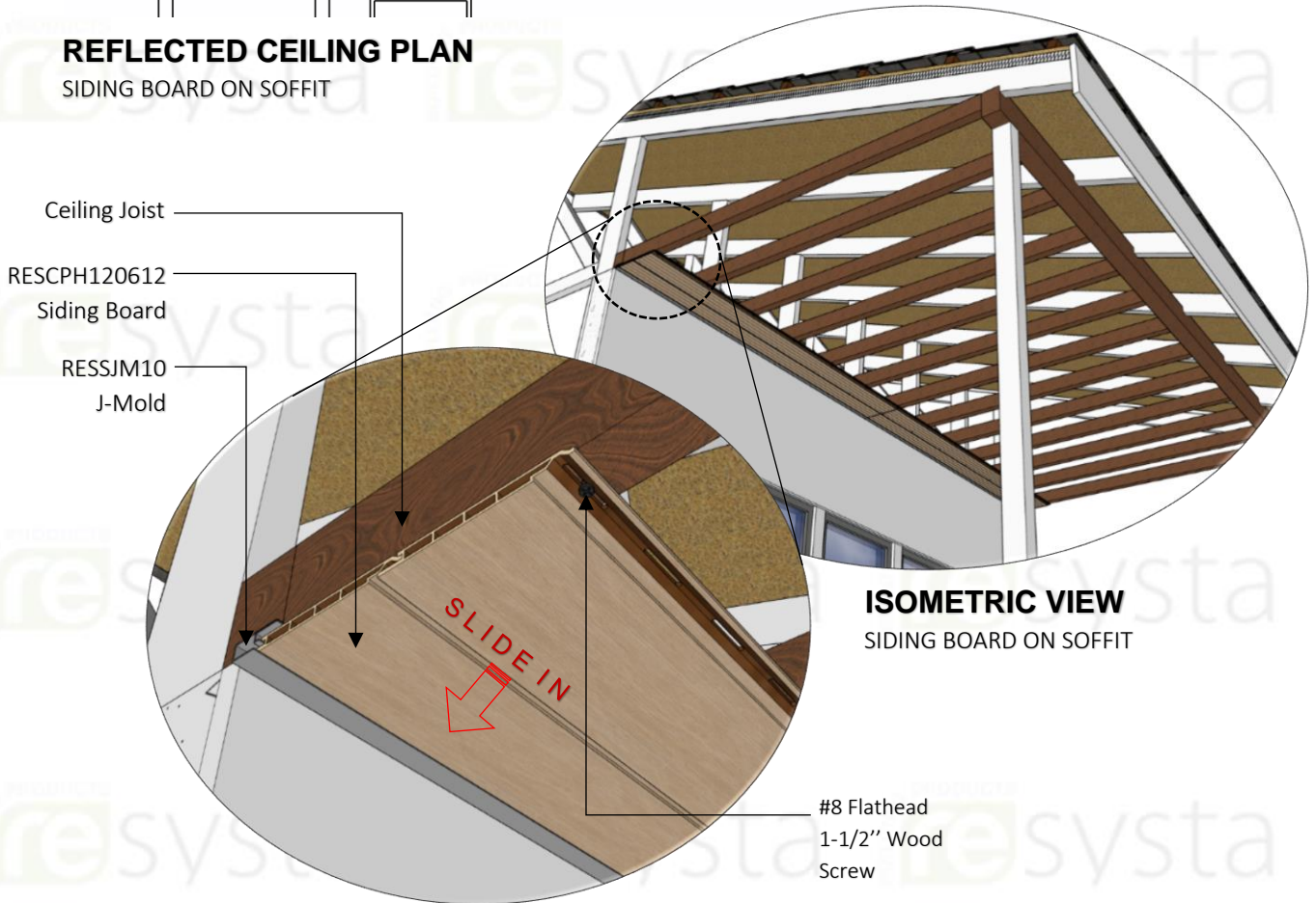
ISOMETRIC DETAIL SIDING BOARD ON SOFFIT
