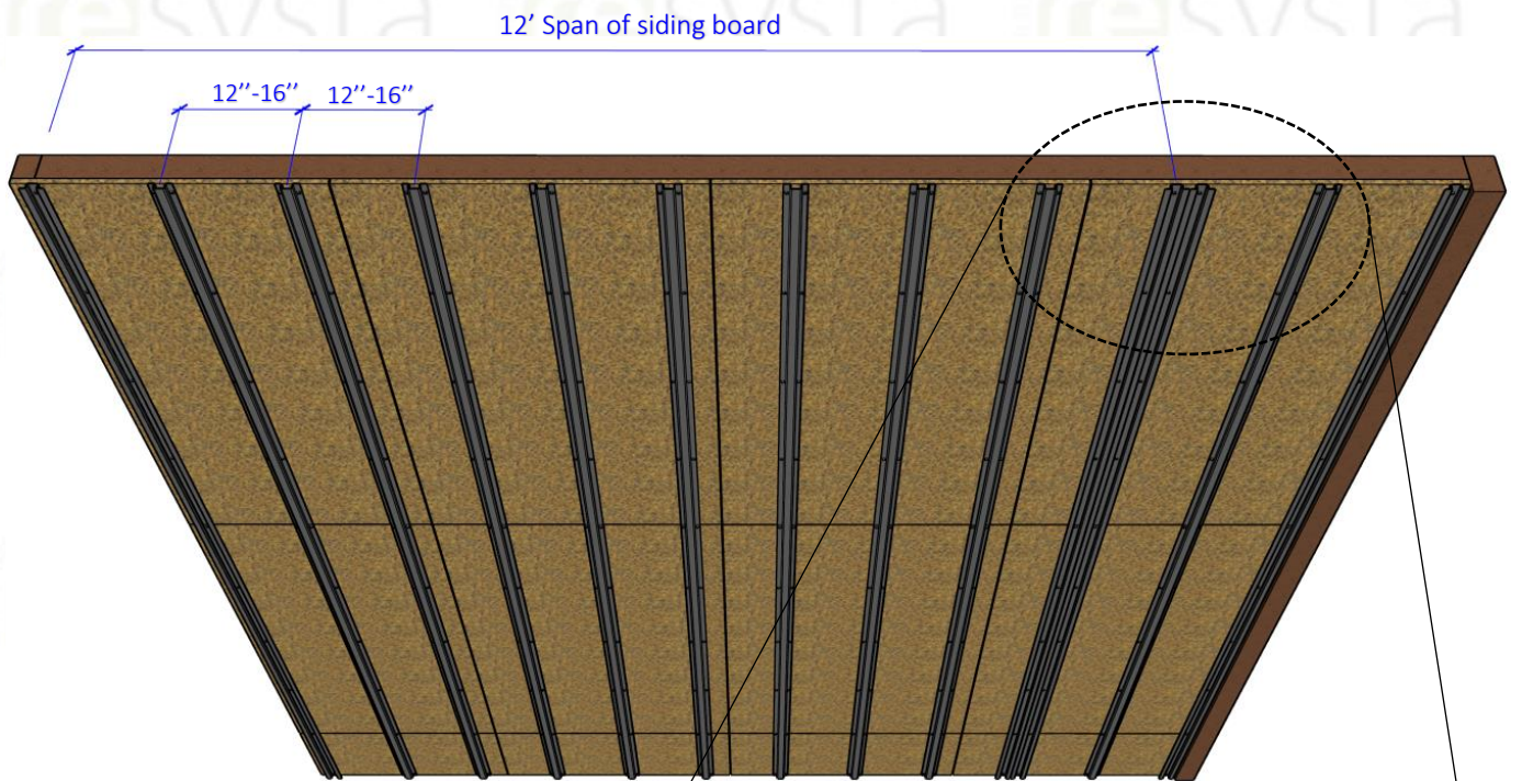
REFLECTED CEILING PLAN BATTENS LAYOUT
