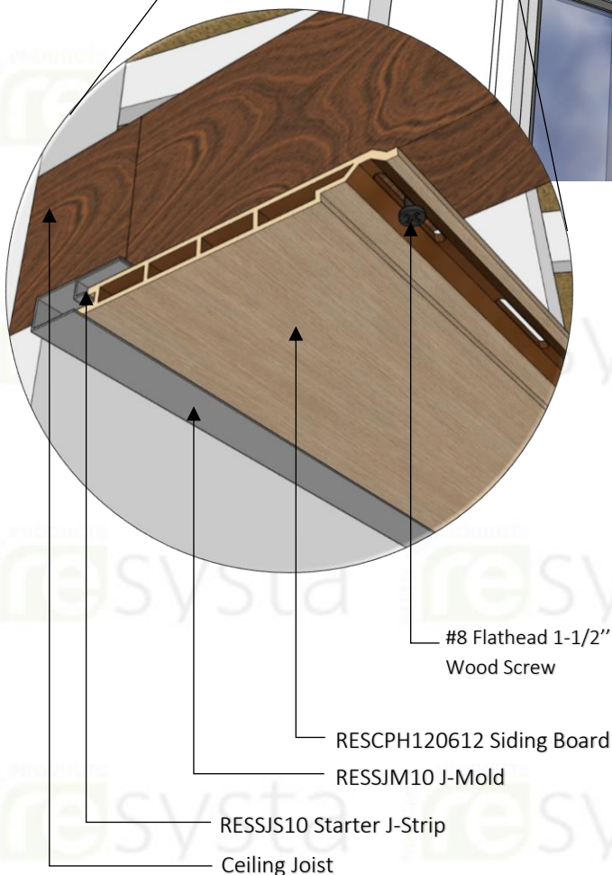
ISOMETRIC DETAIL SIDING BOARD ON SOFFIT
