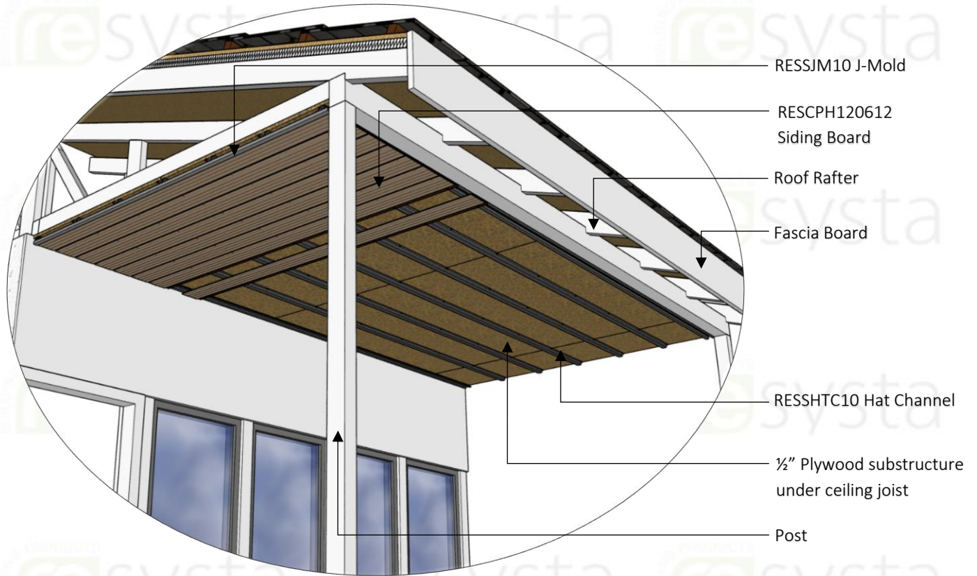
ISOMETRIC VIEW SIDING BOARD ON SOFFIT
