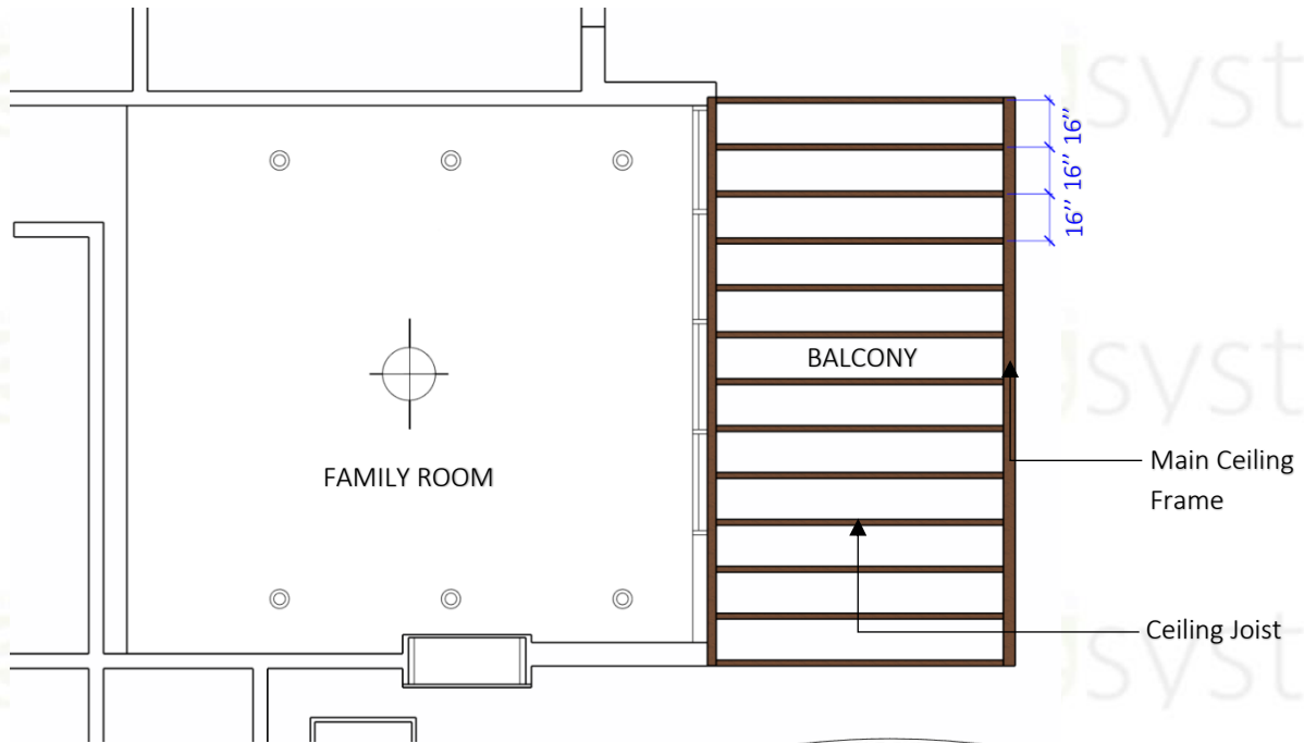
REFLECTED CEILING PLAN CEILING JOIST LAYOUT
