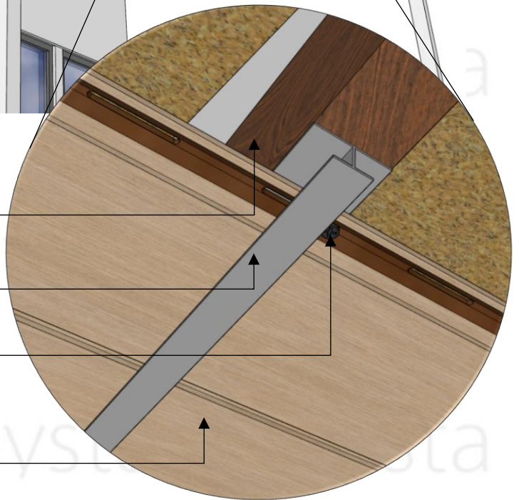
ISOMETRIC VIEW SIDING H-MOLD
