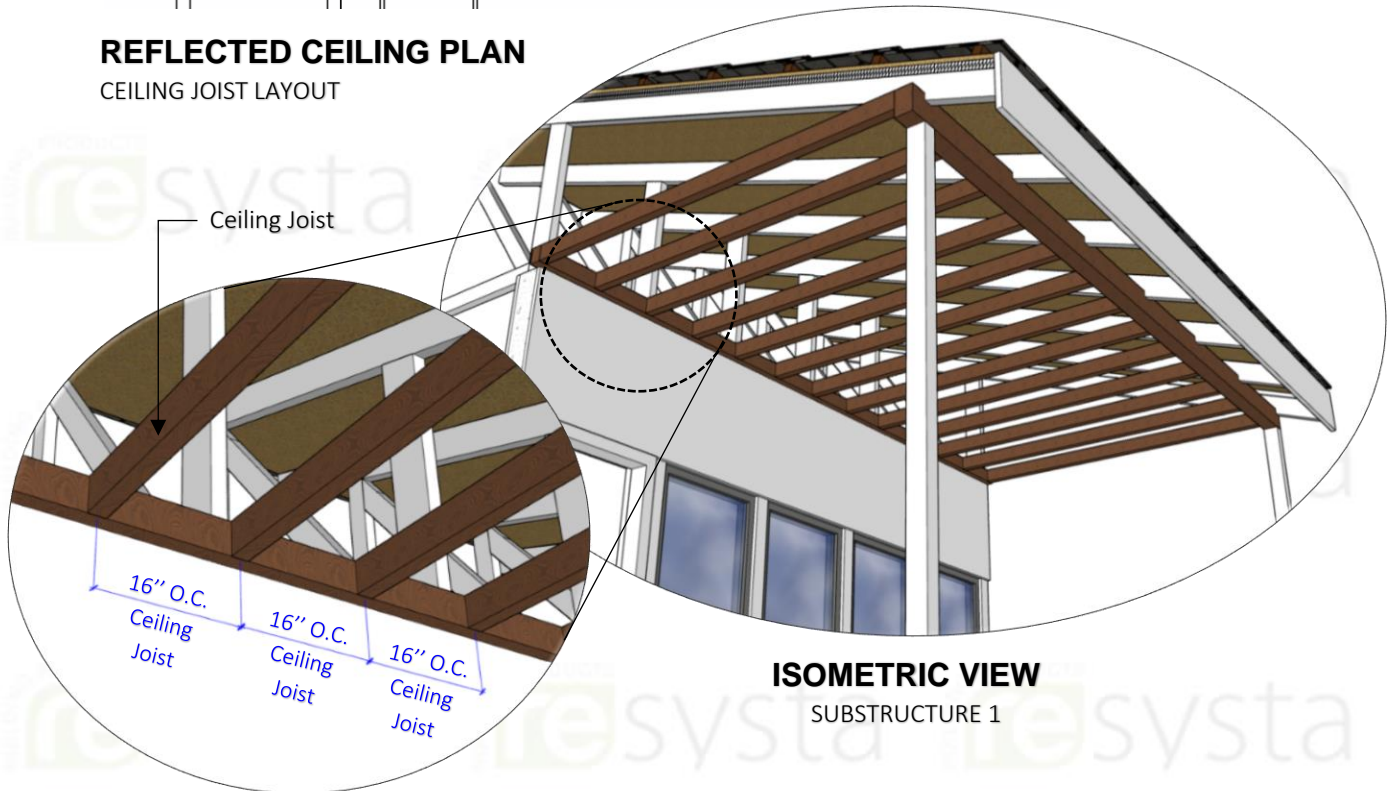
ISOMETRIC DETAIL SUBSTRUCTURE 1
