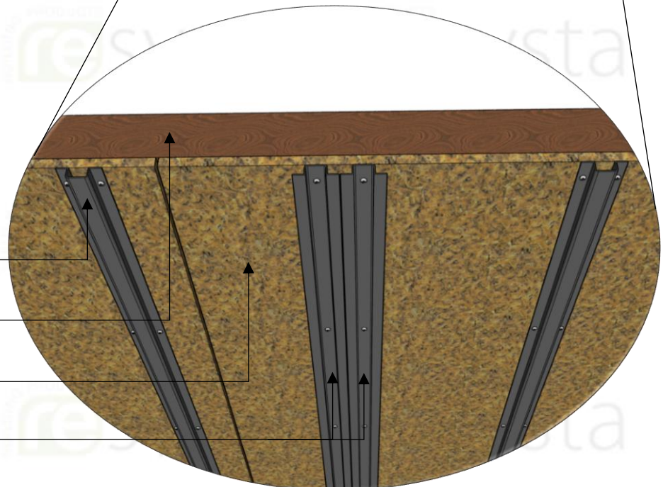
ISOMETRIC DETAIL BATTENS LAYOUT
