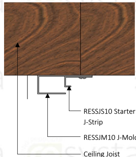
SECTION DETAIL STARTER STRIP AND J-MOLD
