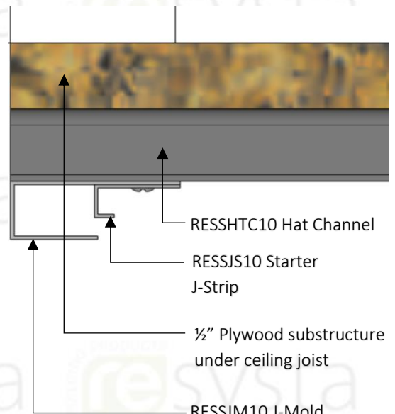
SECTION DETAIL STARTER STRIP AND J-MOLD
