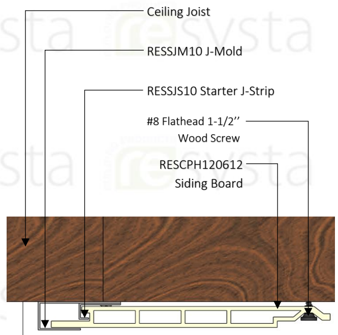
SECTION DETAIL SIDING BOARD ON SOFFIT
