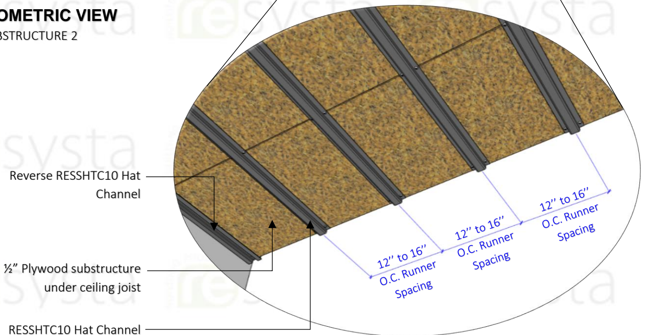
ISOMETRIC DETAIL SUBSTRUCTURE 2
