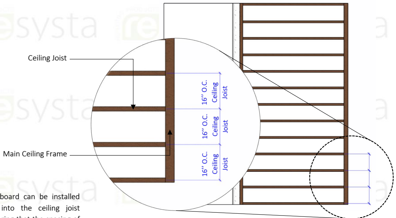
PLAN SUBSTRUCTURE 1
